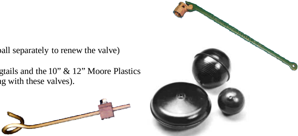
(Copper pigtail passes through center hole of a pan float – connects float to the valve)
